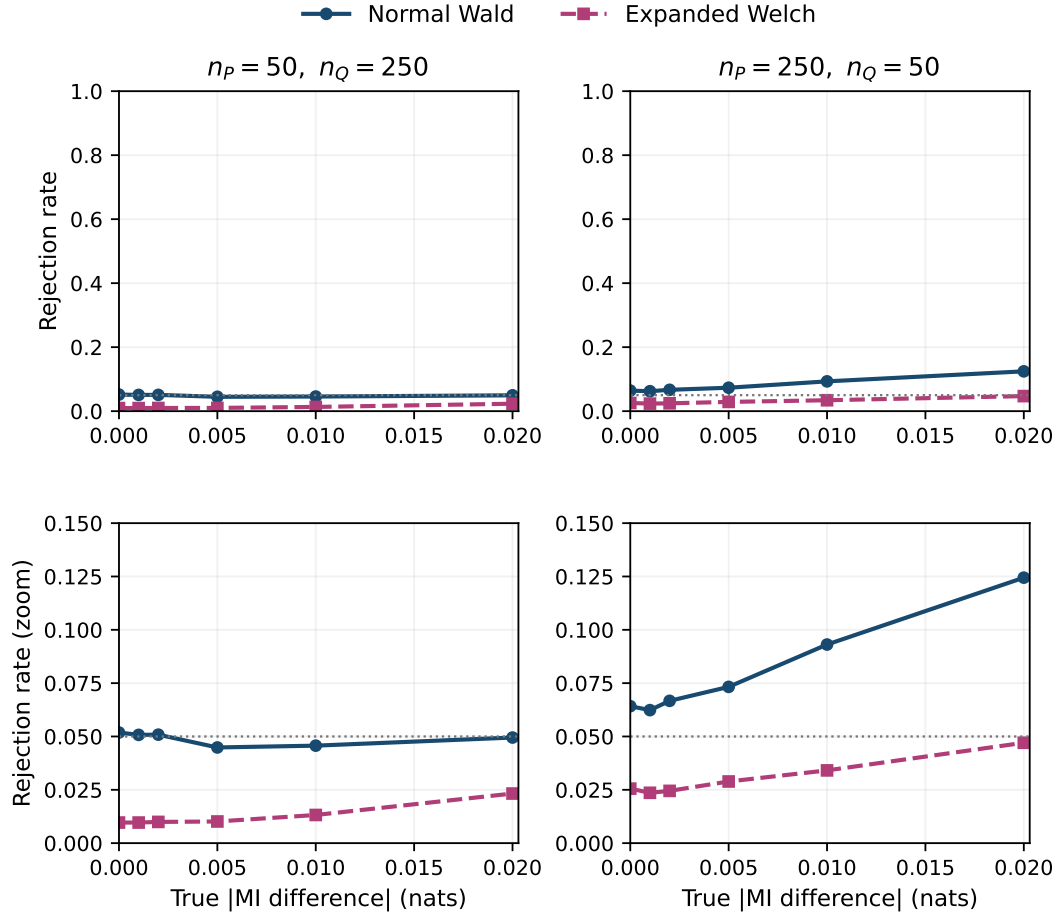
Figure C.5: Rejection rates under two sample allocations when P has the higher MI.
