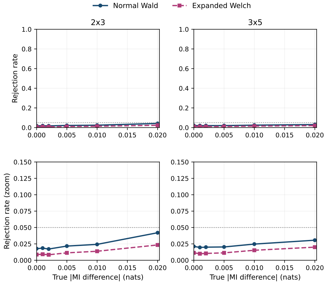
Figure C.6: Rejection rates for 2 \times 3 and 3 \times 5 tables with different margins.
