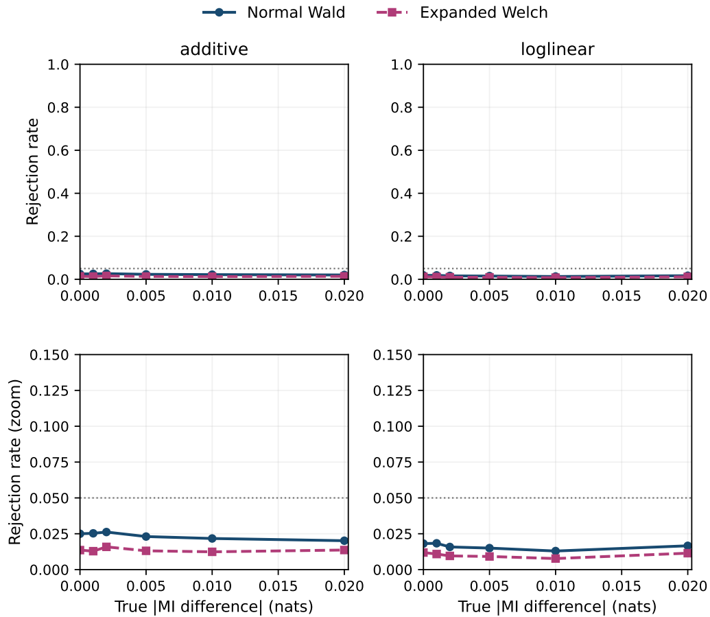
Figure C.7: Rejection rates under additive and ordinal log-linear constructions for 5 \times 5 tables.
