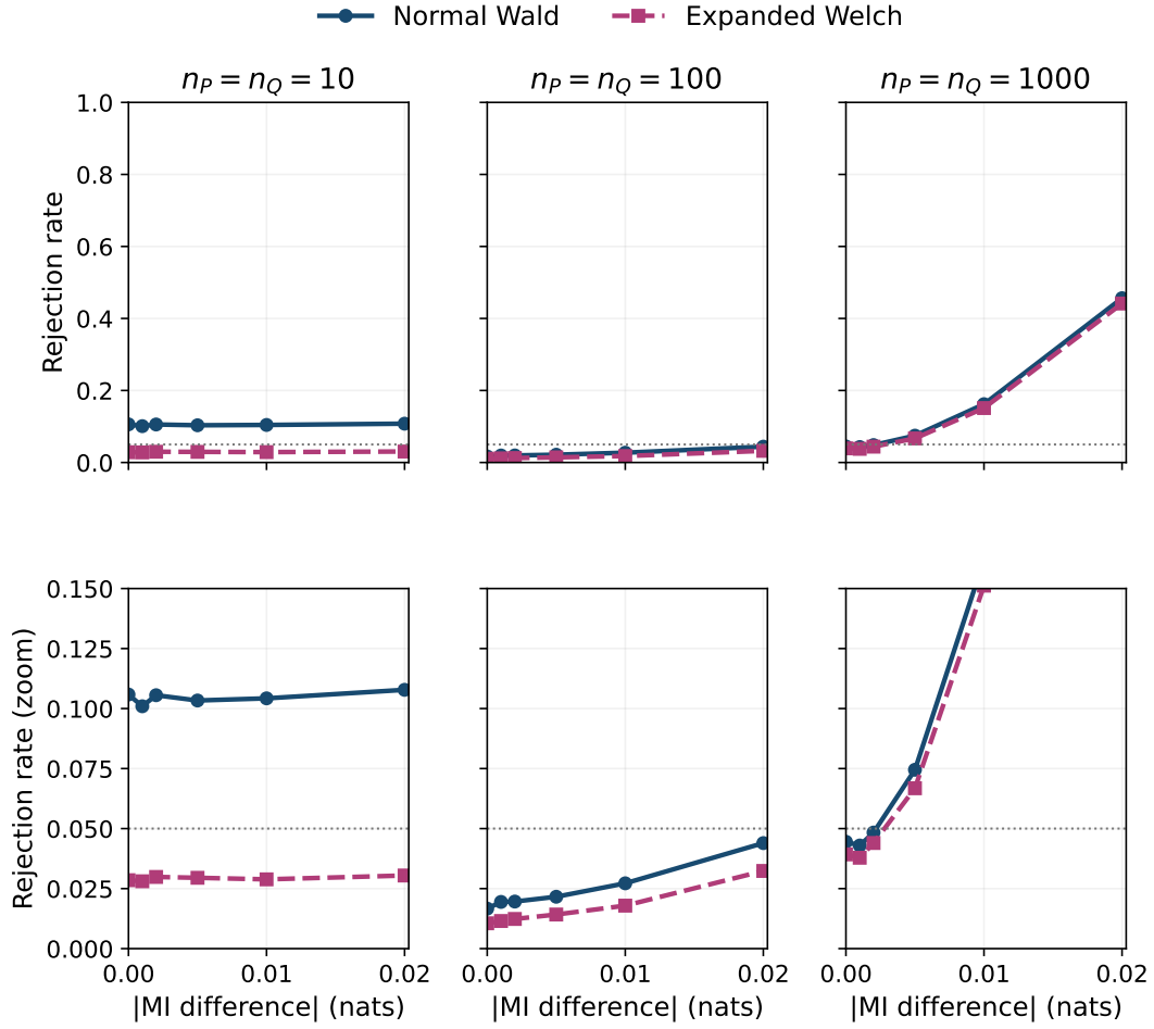
Figure C.1: Normal Wald and Expanded Welch rejection rates for 3 \times 3 tables under the uniform margin profile. The lower panels enlarge the 0–0.15 range.
