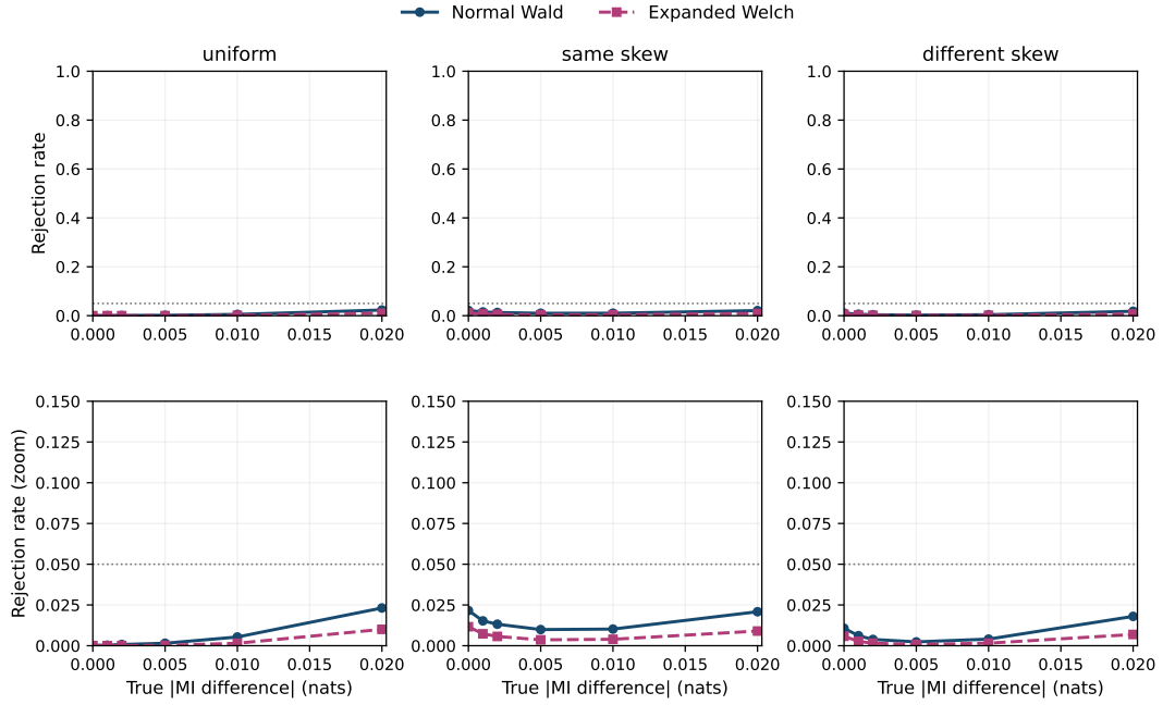
Figure C.8: Rejection rates for 2 \times 2 tables starting at exact independence.
