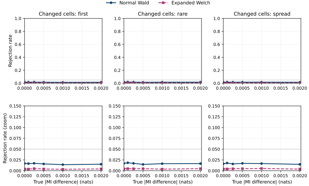
Figure C.3: Rejection rates for 5 \times 5 tables with association in different cells.
