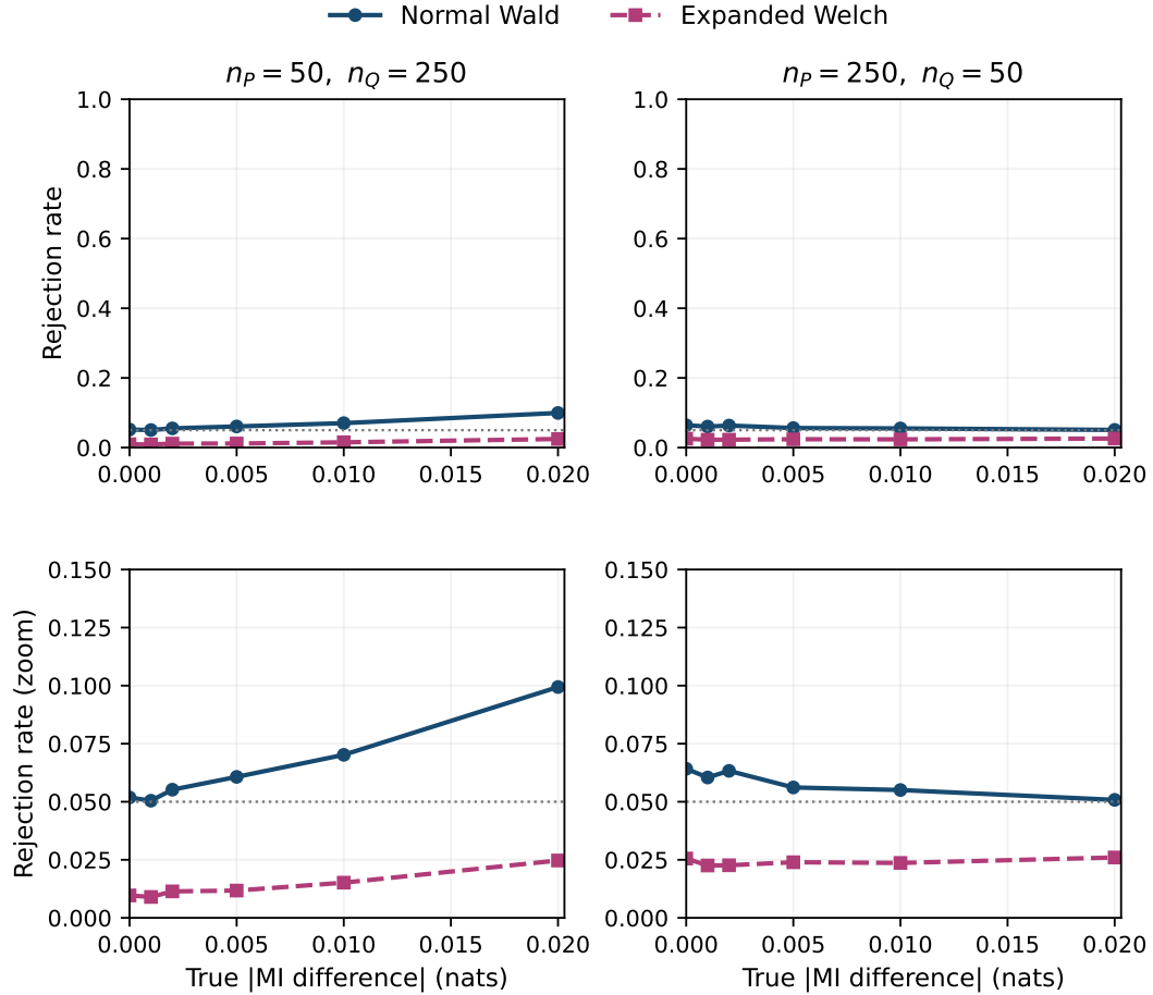
Figure C.4: Rejection rates under two sample allocations when Q has the higher MI.
