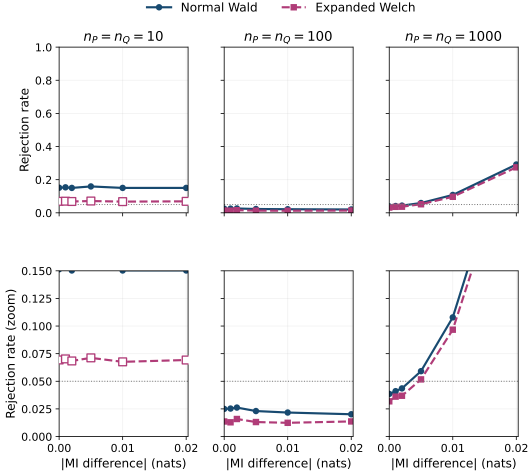
Figure C.2: Normal Wald and Expanded Welch rejection rates for 5 \times 5 tables under the different skew margin profile. The lower panels enlarge the 0–0.15 range.
